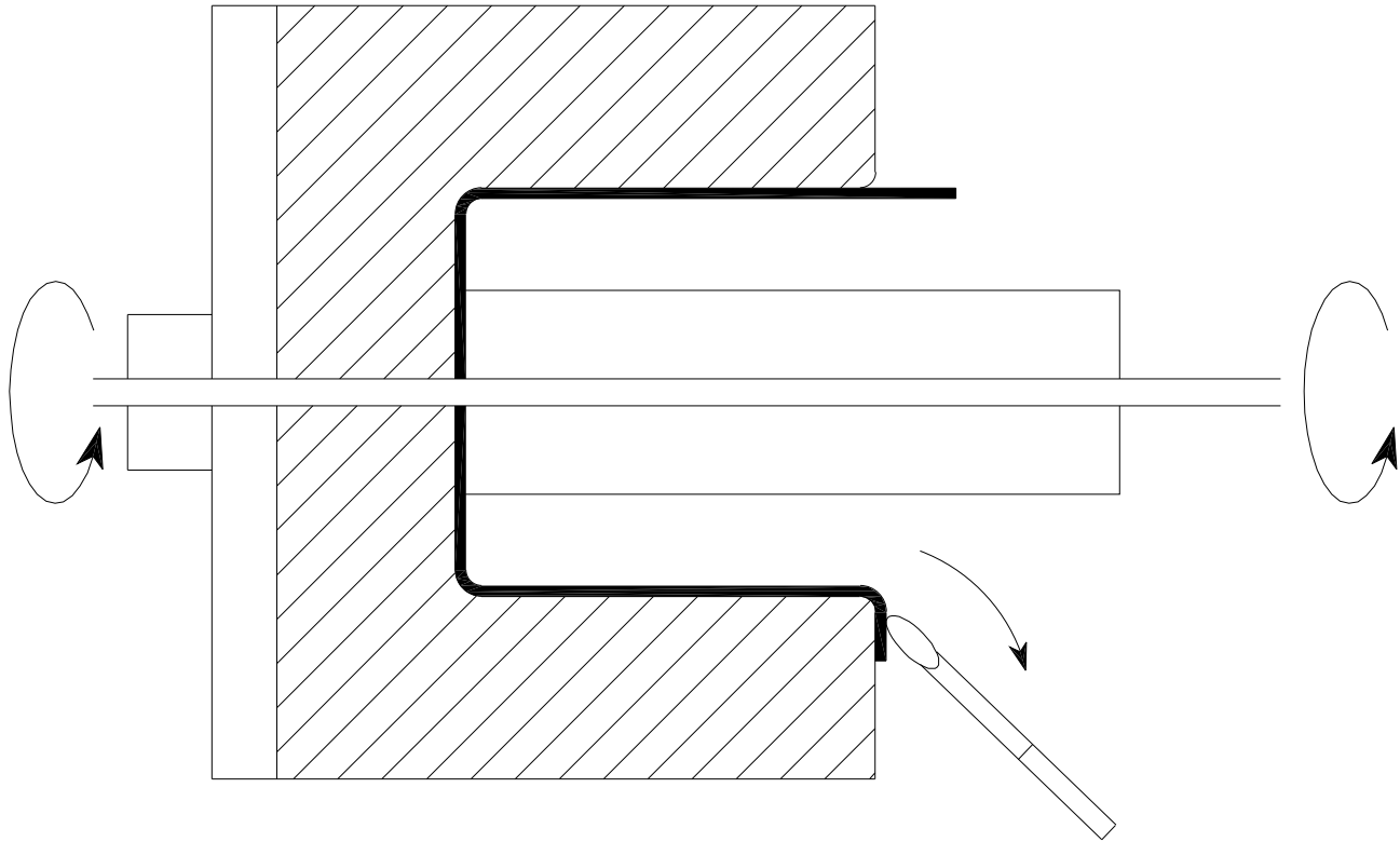
External Flanging
